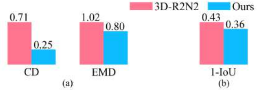
Figure 7. Quantitative comparison to 3D-R2N2. (a) Point-set based metrics CD and EMD. (b) Volumetric representation based metric 1-IoU. Lower bars indicate smaller errors. Our method gives better results on all three metrics.
