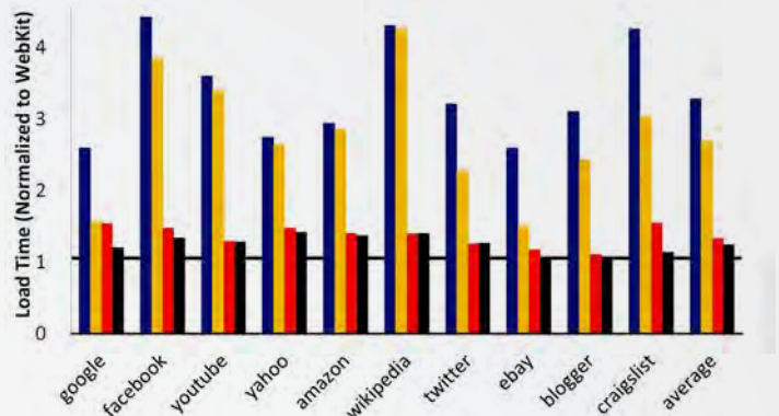
Quark load times for the Alexa Top 10 Web sites, normalized to stock WebKit's load times. In each group the blue bar shows the unoptimized load time, the black bar shows load time in the final, optimized version of Quark, and center bars show how additional optimizations improve performance.
